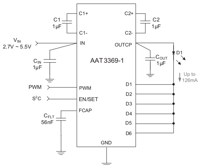
Figure 5: Higher Current, Single LED Application.
