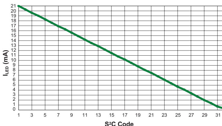
Figure 2: LED Current Controlled by S 2 Cwire Only.
